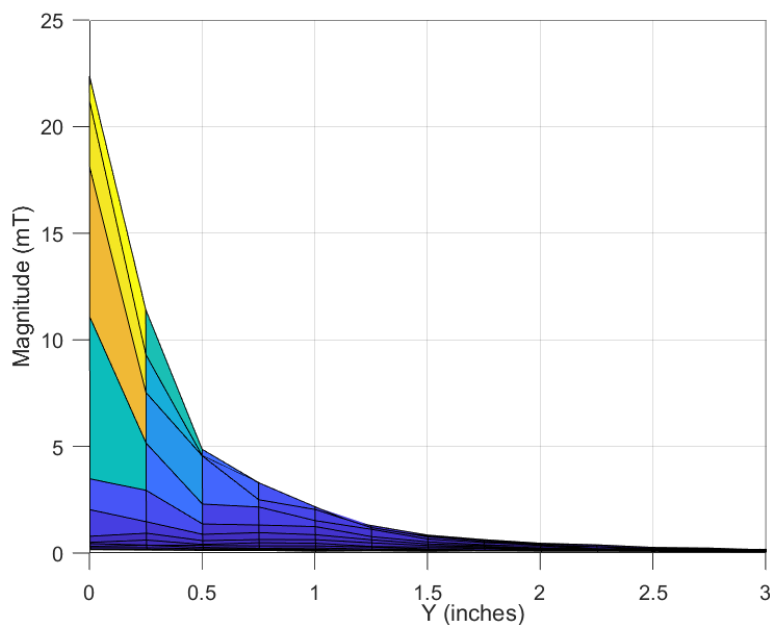
Figure 3-8. TMA5273 Magnet 2 Detection Field (2D)
