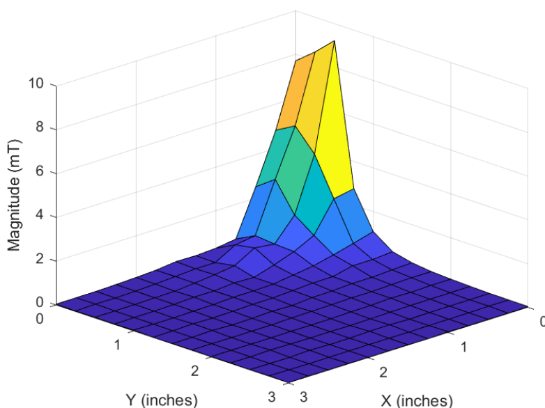
Figure 3-5. TMAG5273 Magnet 1 Detection Field (3D)
