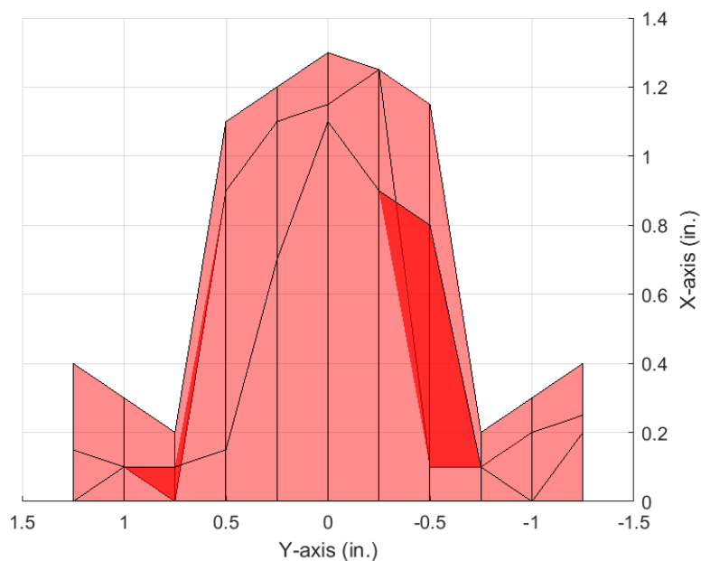
Figure 3-10. Reed Switch Magnet 2 Detection Field (2D Top Down)
