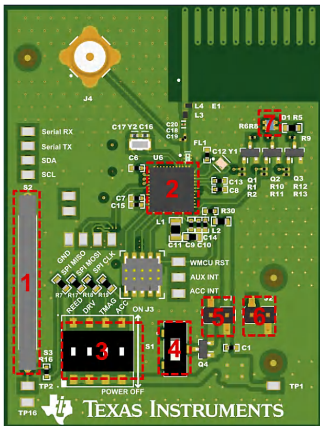
Figure 2-2. Door and Window Sensor Evaluation Platform Top View
