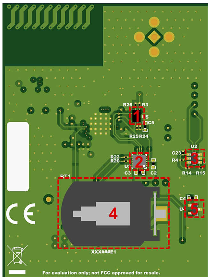
Figure 2-3. Door and Window Sensor Evaluation Platform Bottom View
