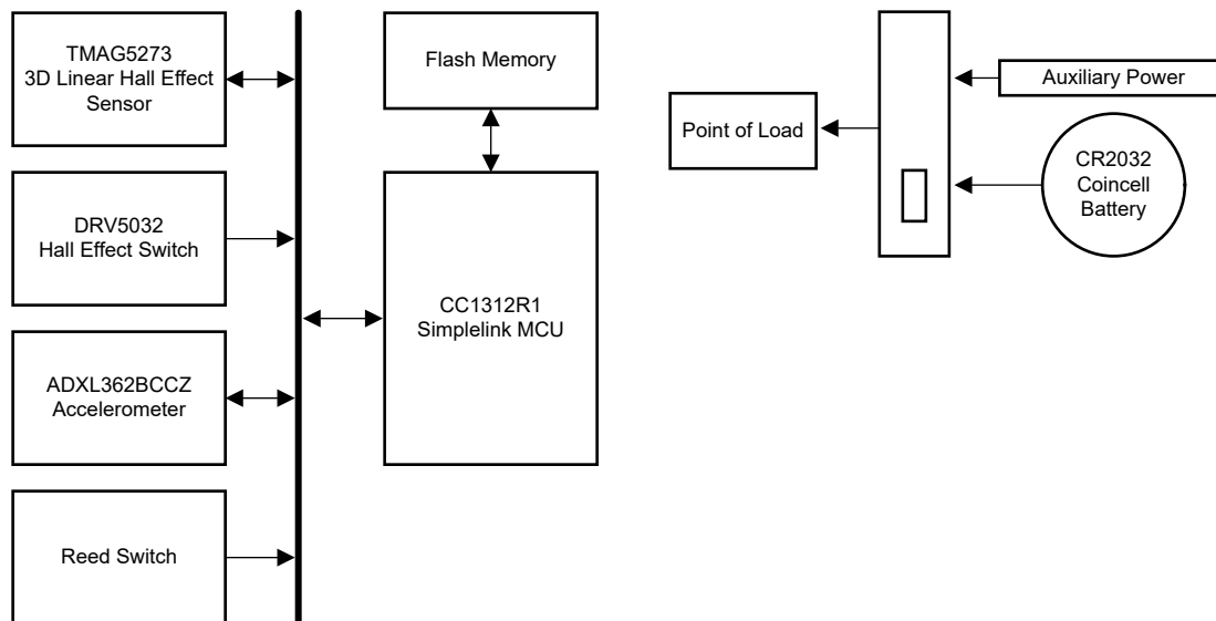
Figure 2-1. Block Diagram
