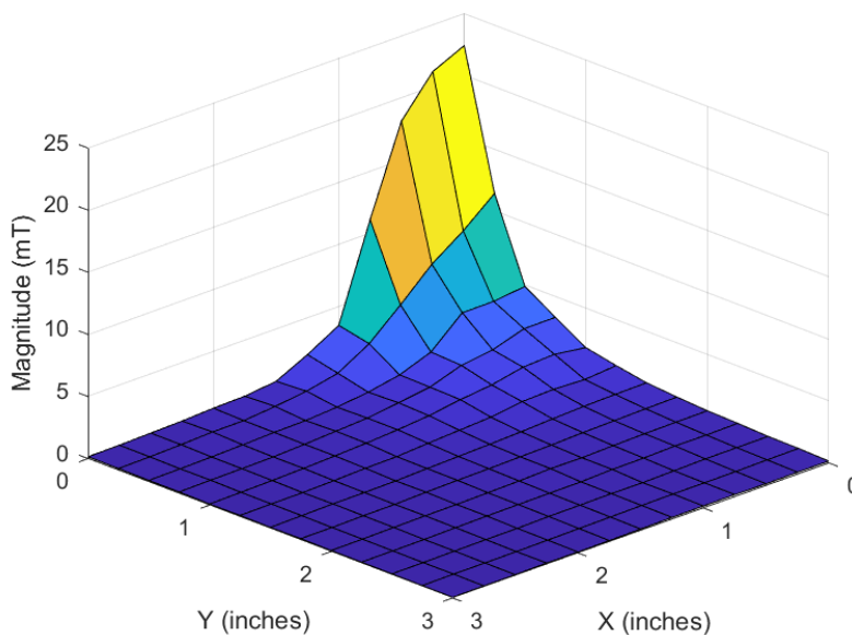
Figure 3-9. TMA5273 Magnet 2 Detection Field (3D)
