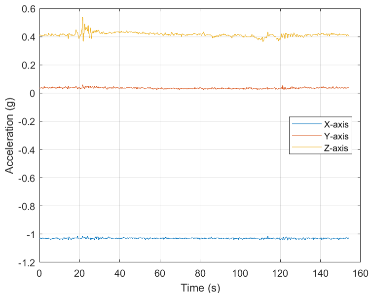
Figure 3-12. Accelerometer Door Open Event
