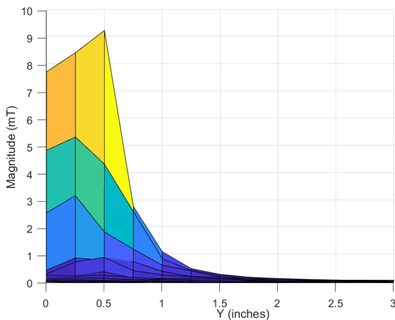
Figure 3-4. TMAG5273 Magnet 1 Detection Field (2D)
