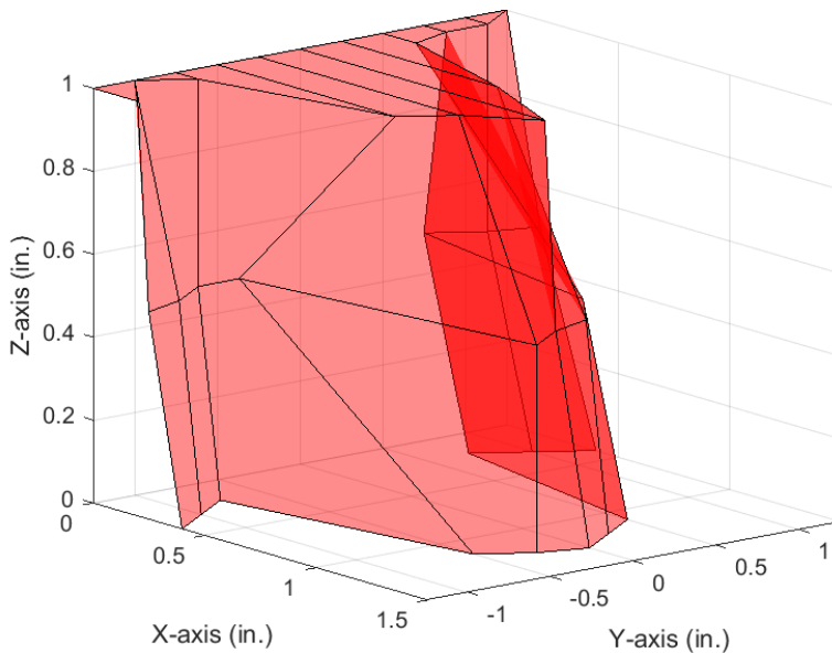
Figure 3-11. Reed Switch Magnet 2 Detection Field (3D)
