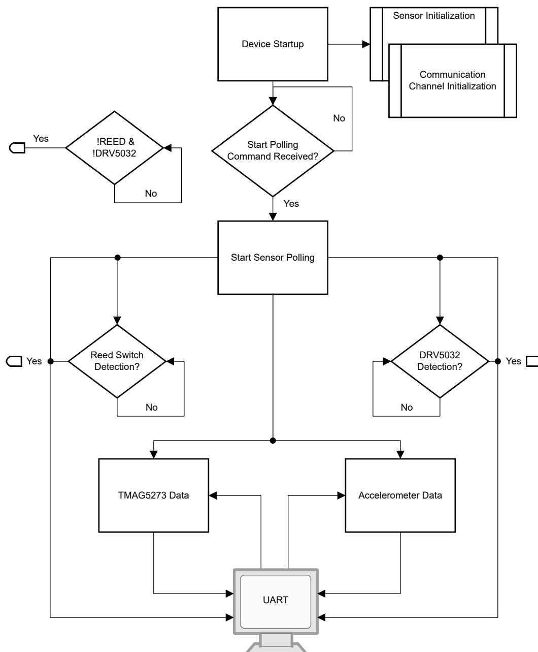
Figure 3-3. Software Flowchart
