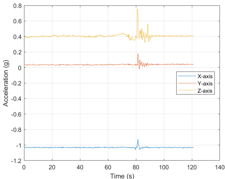
Figure 3-13. Accelerometer Door Close Event
