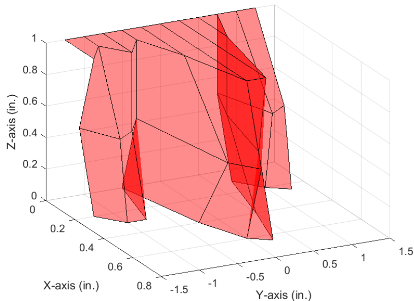
Figure 3-7. Reed Switch Magnet 1 Detection Field (3D)
