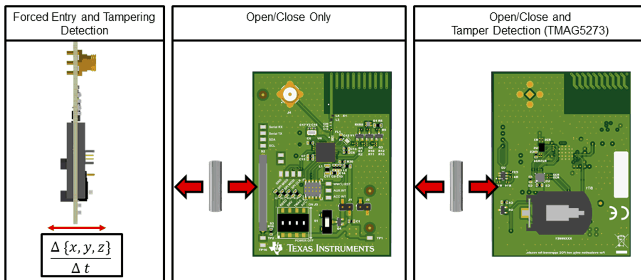
Figure 2-4. Event Detection Modes
