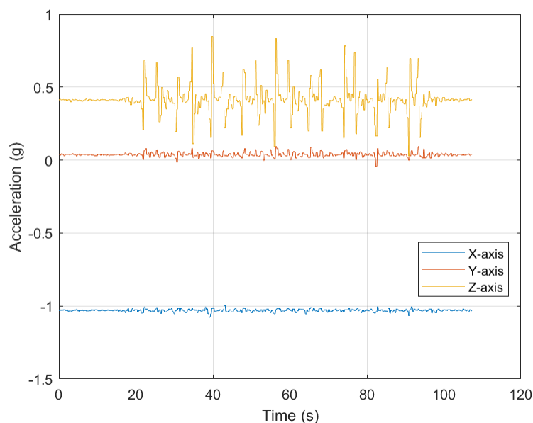
Figure 3-14. Accelerometer Brute Force Entry Attempt
